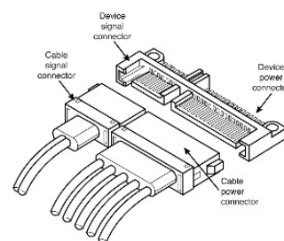
Figure 3. Attaching SATA cabling
